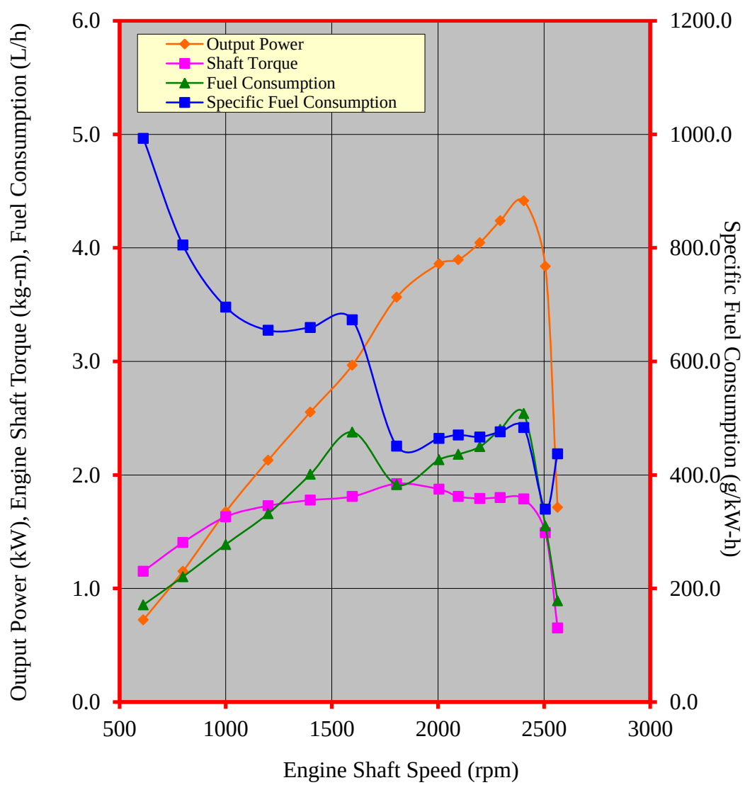
Figure 3. Performance characteristic curves of the KUVICO KV70 diesel engine
