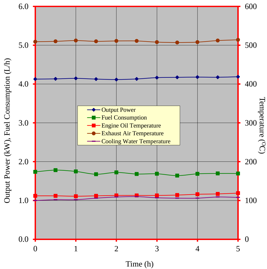
Figure 4. Performance characteristic curves during the continuous running test of the KUVICO KV70 diesel engine
